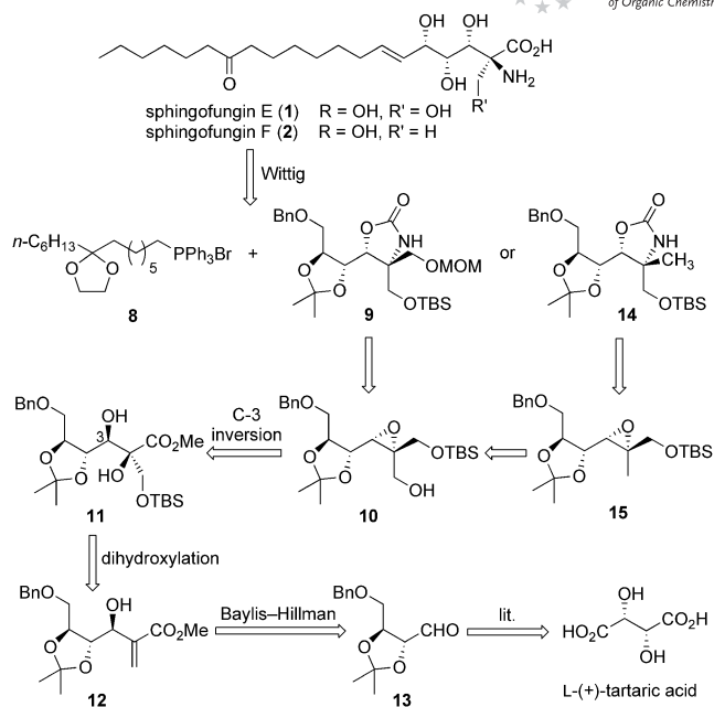
Scheme 1. Retrosynthetic analysis of sphingofungins E ( 1 ) and F ( 2 ).
