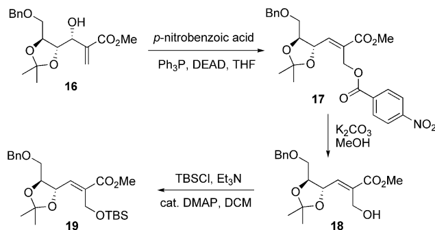
Scheme 3. Transformations of minor Baylis–Hillman adduct 16 .
