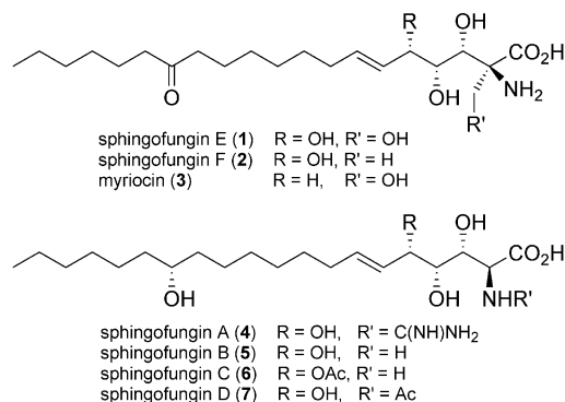
Figure 1. Sphingofungin E and F and related natural products.
