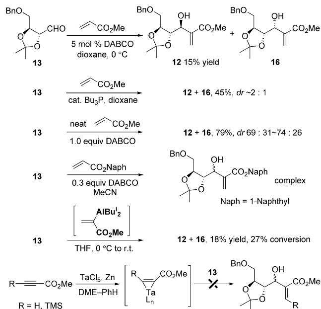
Scheme 2. Attempted optimization of the Baylis–Hillman reaction of 13 .
