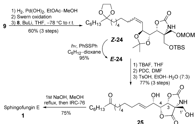
Scheme 5. Synthesis of sphingofungin E ( 1 ).
