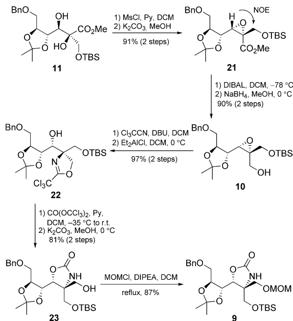
Scheme 4. Elaboration of the polar “head” segment.
